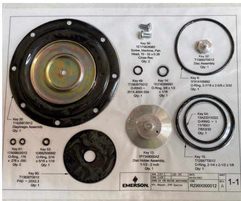
Fisher 299HX Code: 180098
